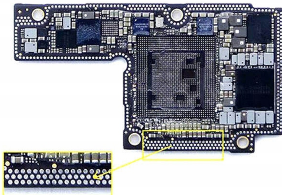
After repair solder points
