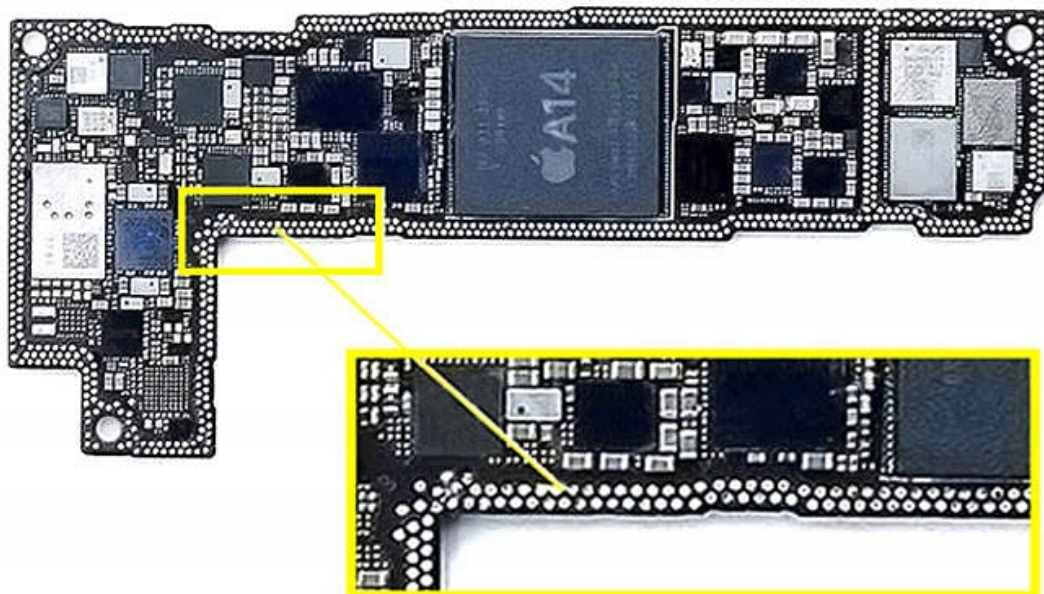
After repair solder points
