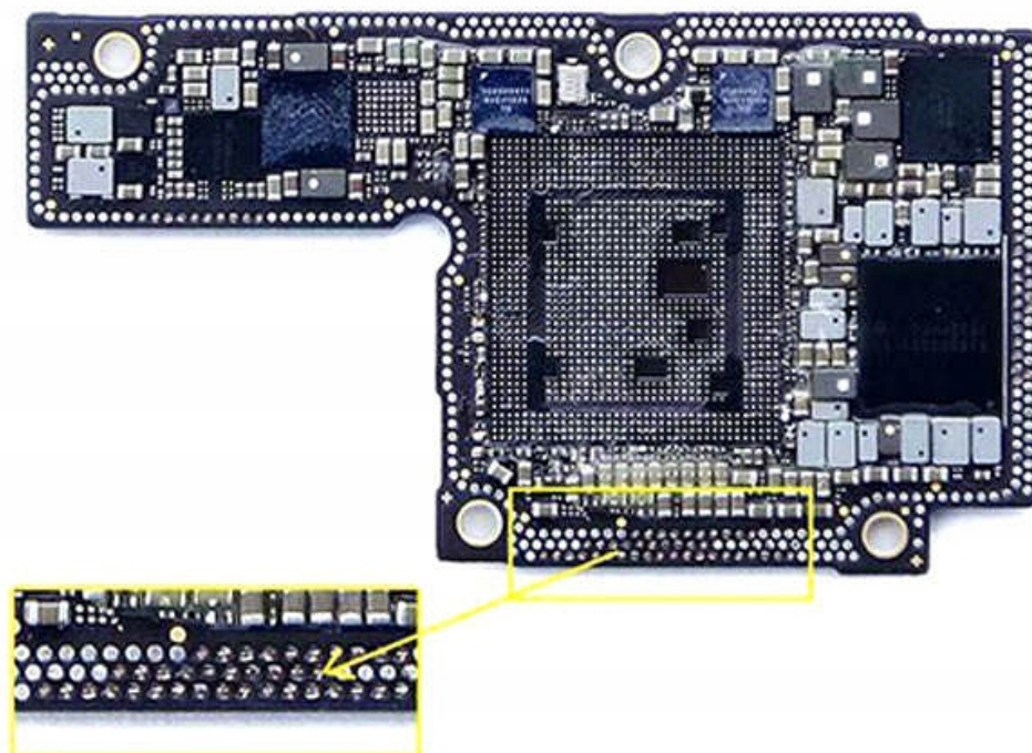
Before repair solder points
